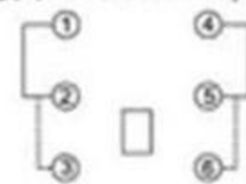
SCHEMATIC (NON-SHORTING)
